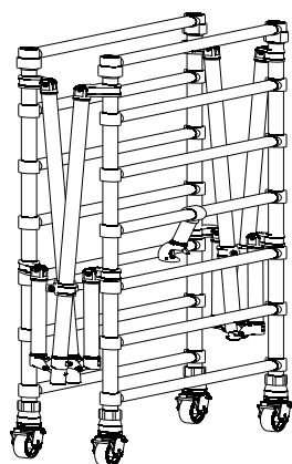
Double Base Frames
