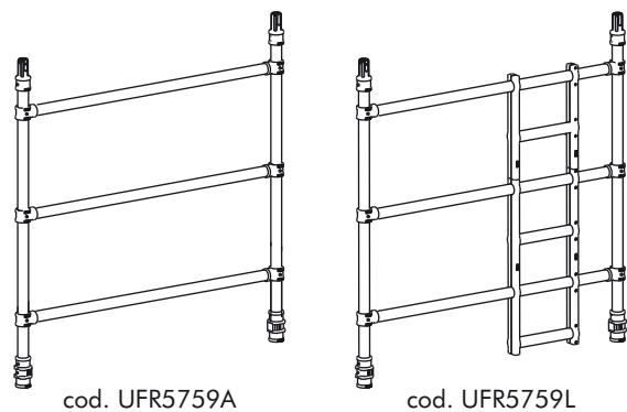
Cadres doubles 1,50m/3rung:
